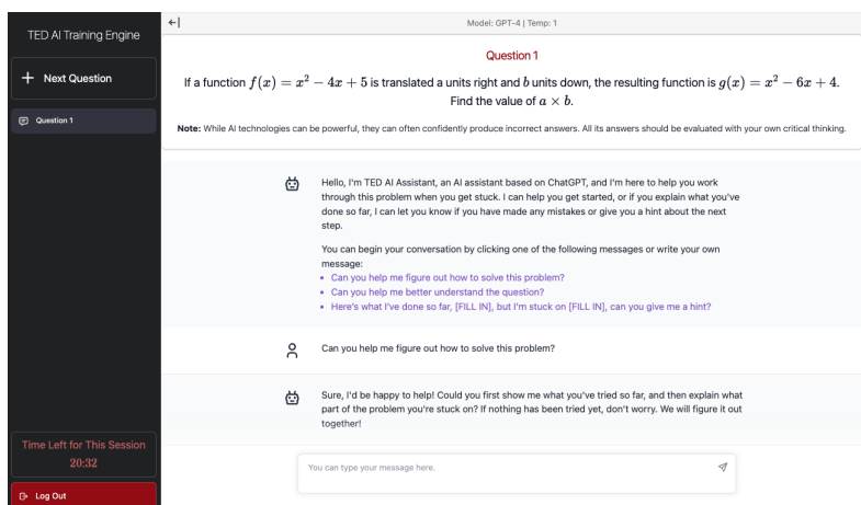
Figure 4: Screen shot of different steps in using our GPT Base and GPT Tutor tools. The tools are identical except for the prompt used in the chat interface.
