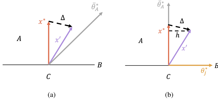
Figure 4: Illustrations for proof sketch of the optimal action gap \nu_* .
