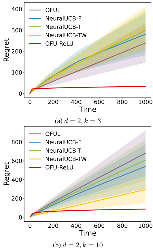
Figure 2: Cumulative regret of a time horizon T = 1,000 over 50 trials with 95% confidence interval.
